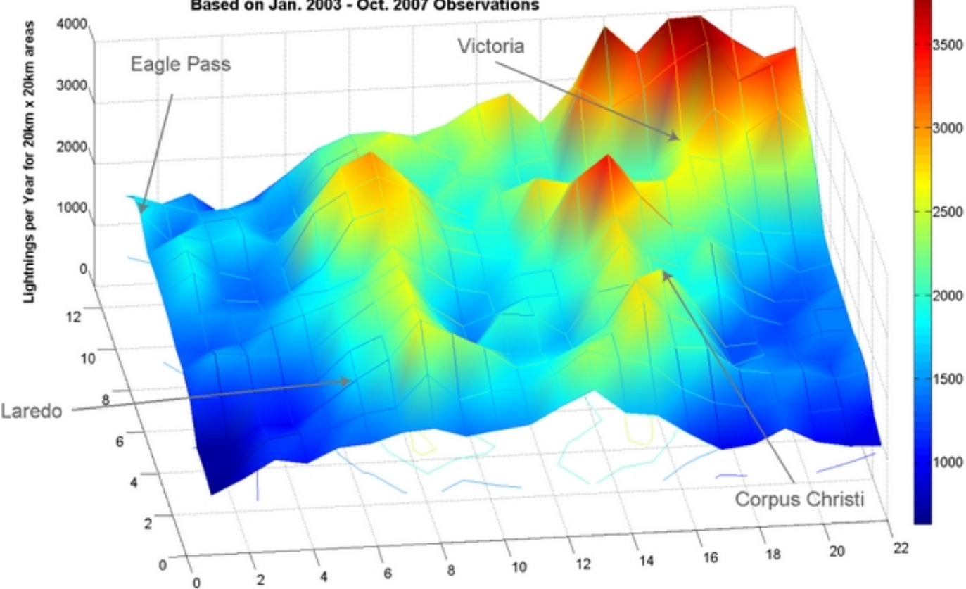
Yearly Lightning Density for the Study Area Based on Jan. 2003 - Oct. 2007 Observations
